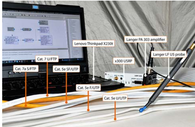
Figure 2: Lab environment including the cables under test, the Universal Software Radio Peripheral (USRP) and the H-field probe.
