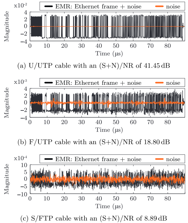
Figure 7: Observed waveforms of the same Ethernet frame and noise. Due to shielding, the signal amplitude reduces which results in decreased signal-to-noise ratios.
