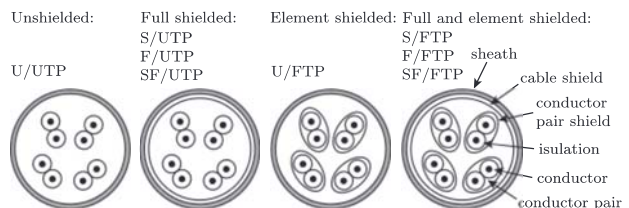
Figure 3: Differently shielded twisted-pair cables
