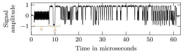
Figure 6: Received frame after down-conversion with f_c = 10 MHz. The preamble with SFD is clearly visible on the left ( \alpha ), followed by the MAC address 00:00:FF:00:00:00 ( \beta ).
