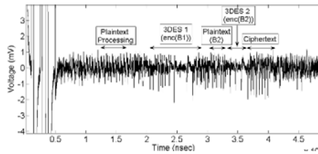
Fig. 12. Overview over operations in amplitude-demodulated trace
