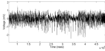
Fig. 6. Demodulated trace (50 kHz - 2 MHz) with analogue filter
