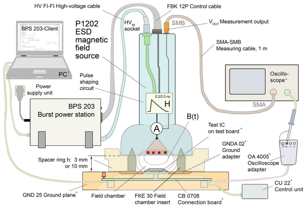
Measurement assembly with P1202 L-ESD (The devices marked * are not included in the scope of delivery.)
