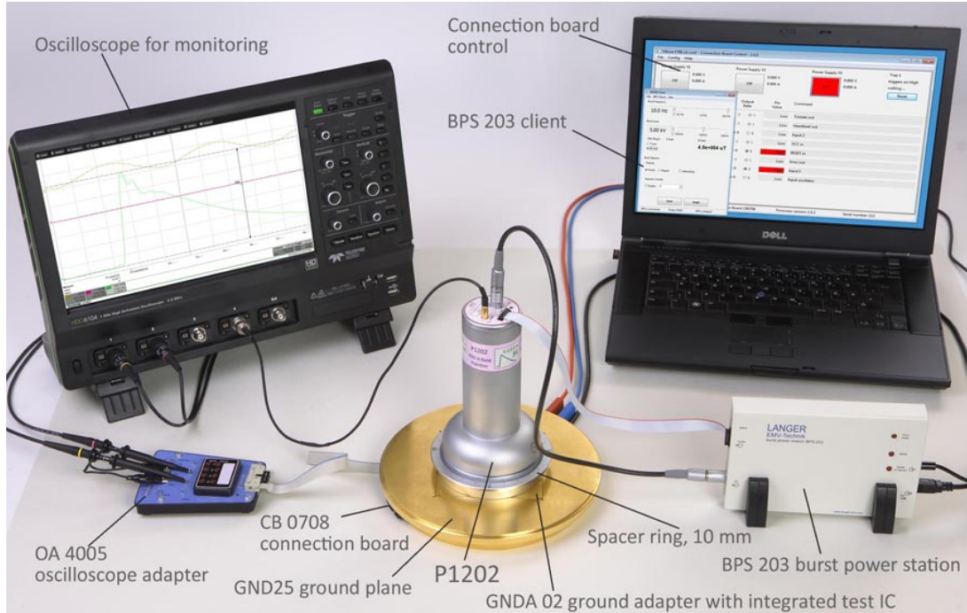
Measurement set-up with P1202 L-ESD Magnetic Field Source Langer Pulse 0.2/2.5 ns
