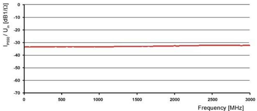
Current transferred by P550 measured on a load of 1 Ohm
