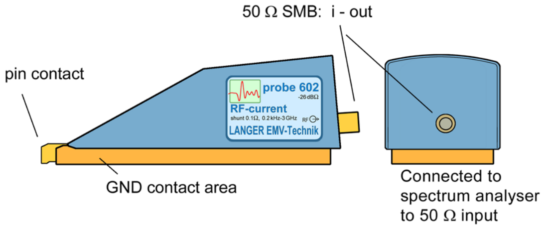
Design, view 1
