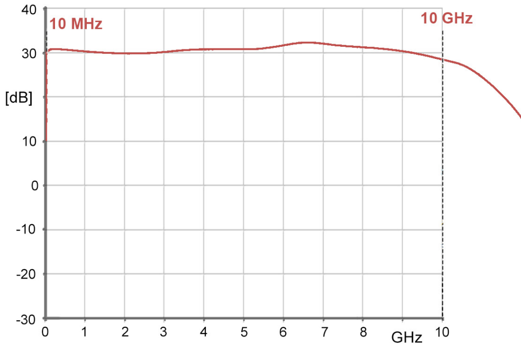
Frequency response
