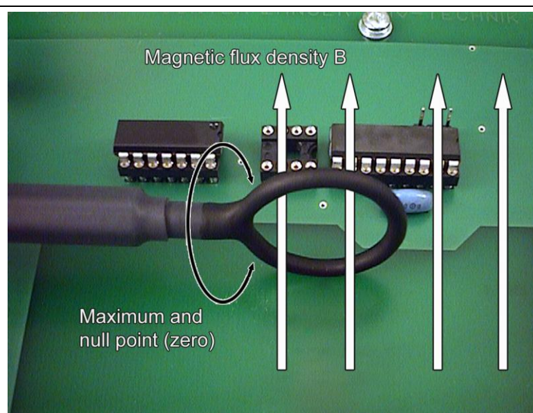
Figure 5 Handling of MS 101 magnetic field probe
