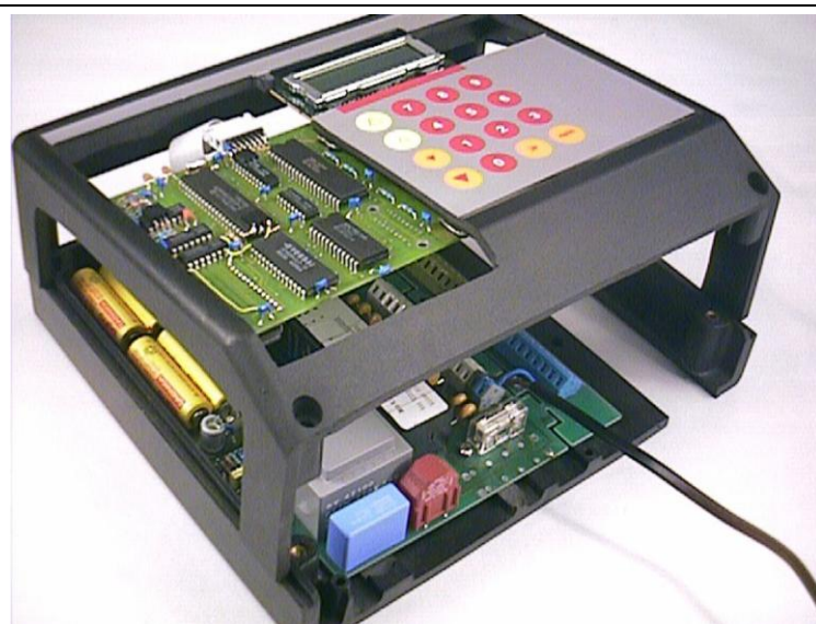
Figure 11 If necessary, special openings must be made in the equipment case so that the measurement areas can be accessed with the probe.
