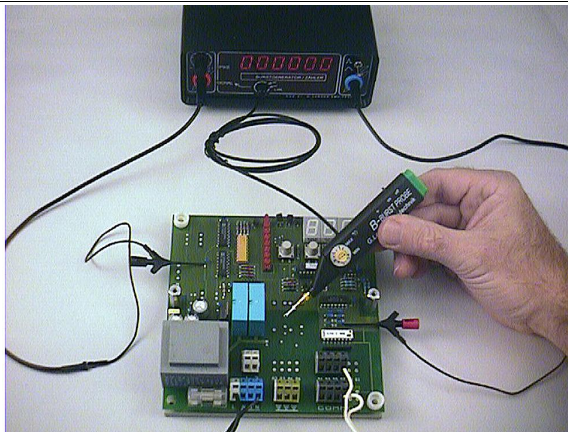
Figure 10 Measuring station for pulse rate procedure
