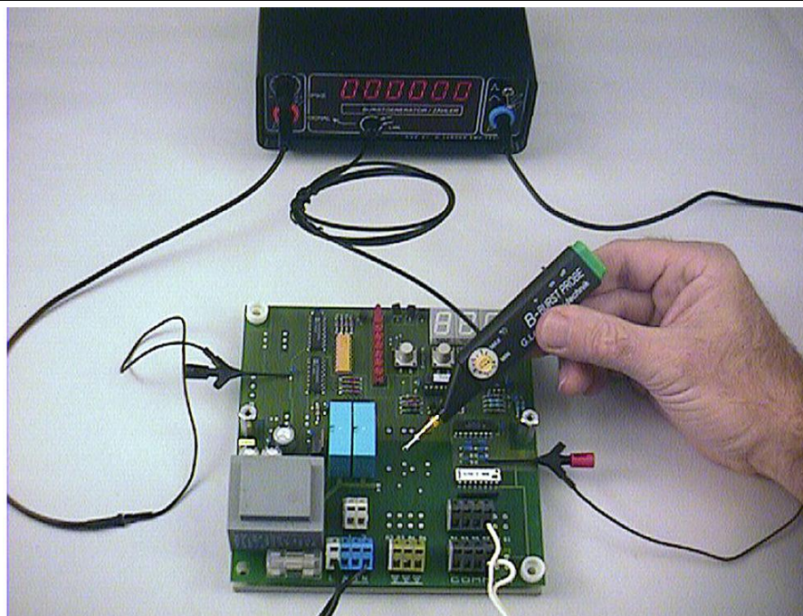
Figure 1 Pulse rate procedure with SGZ 21 burst generator and MSA 02
