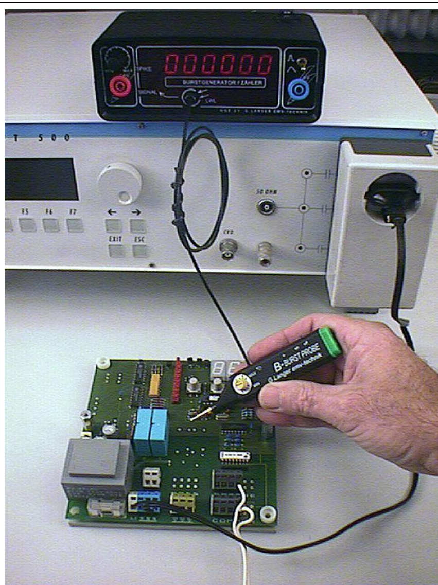
Figure 2 Threshold procedure with MSA 02, SGZ 21 and EFT burst generator according to EN 61000-4-4
