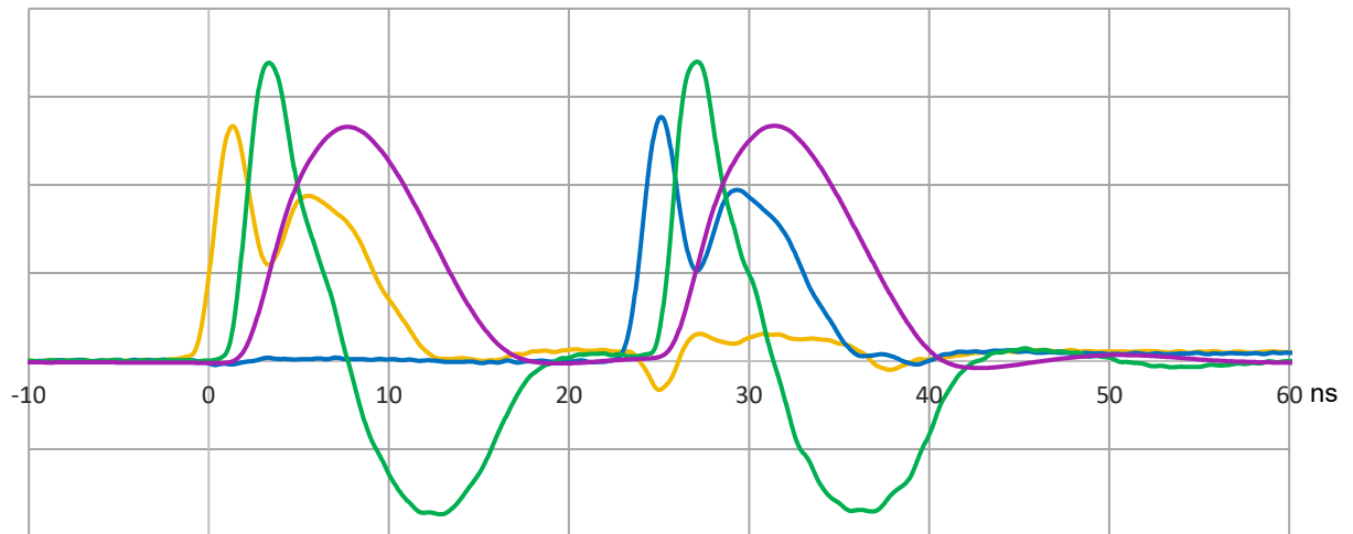
Figure 24: Typical time signals of the ICI-DP HH500-15 in double pulse mode.
