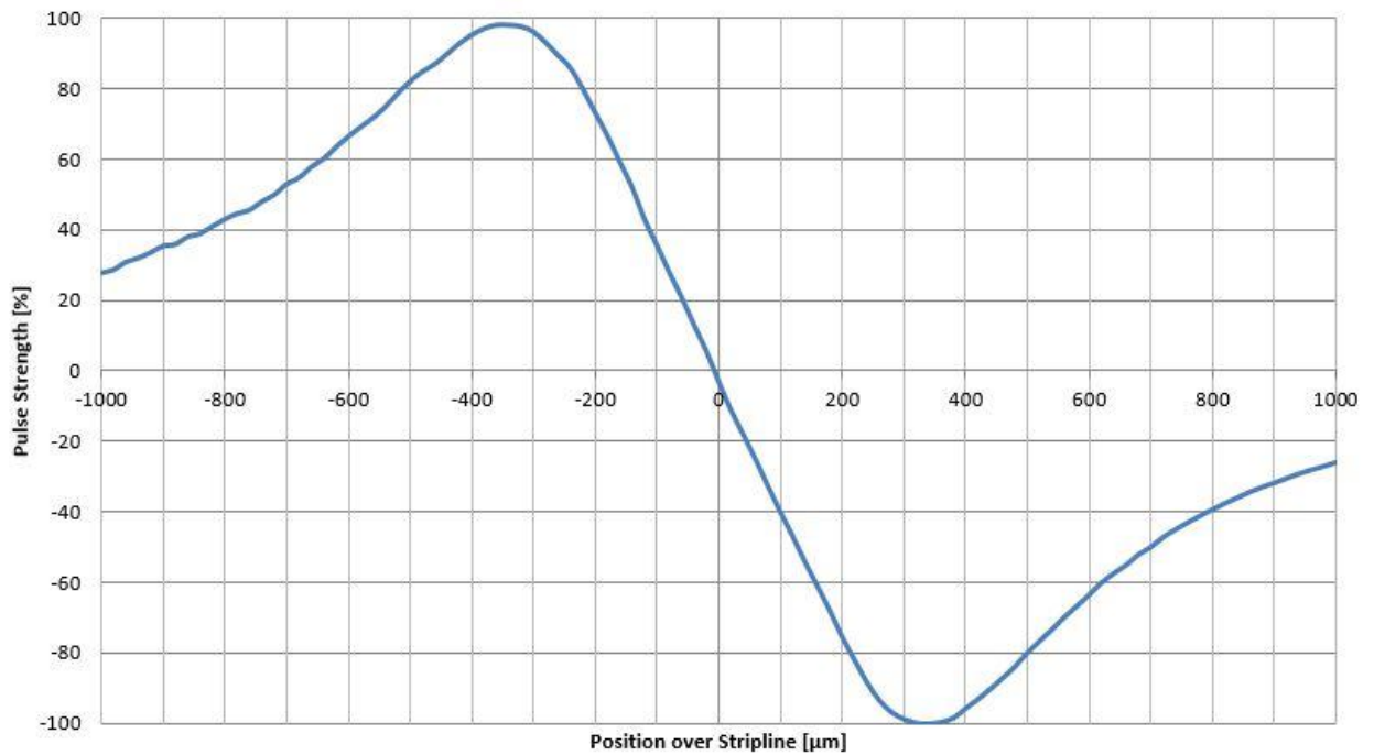
Figure 25: Relative pulse amplitude of the ICI-DP HH500-15 probe in a transverse scan over a 100 \mu\text{m} stripline.
