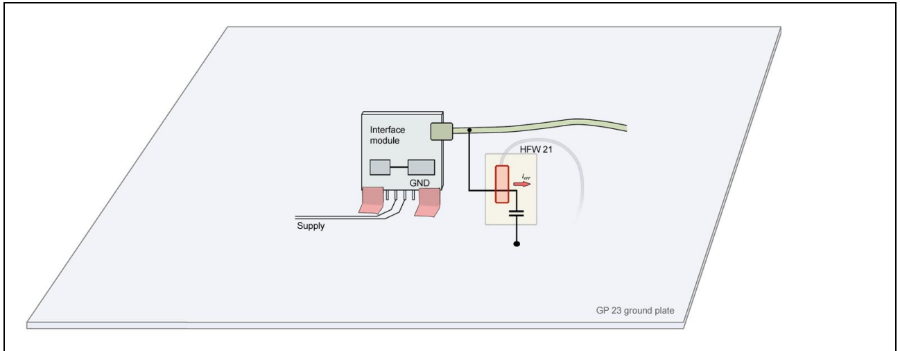
Figure 33 Set-up without the basic unit
