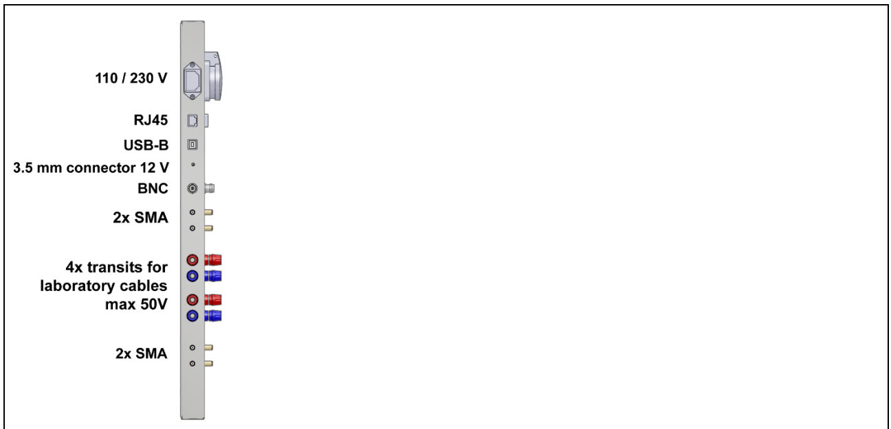
Figure 5 Connections/transits of GP 23 Ground Plate
