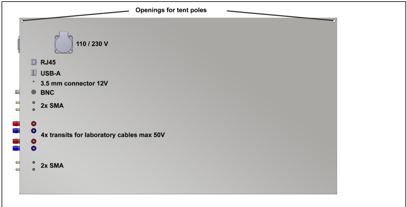
Figure 4 GP 23 Ground Plate
