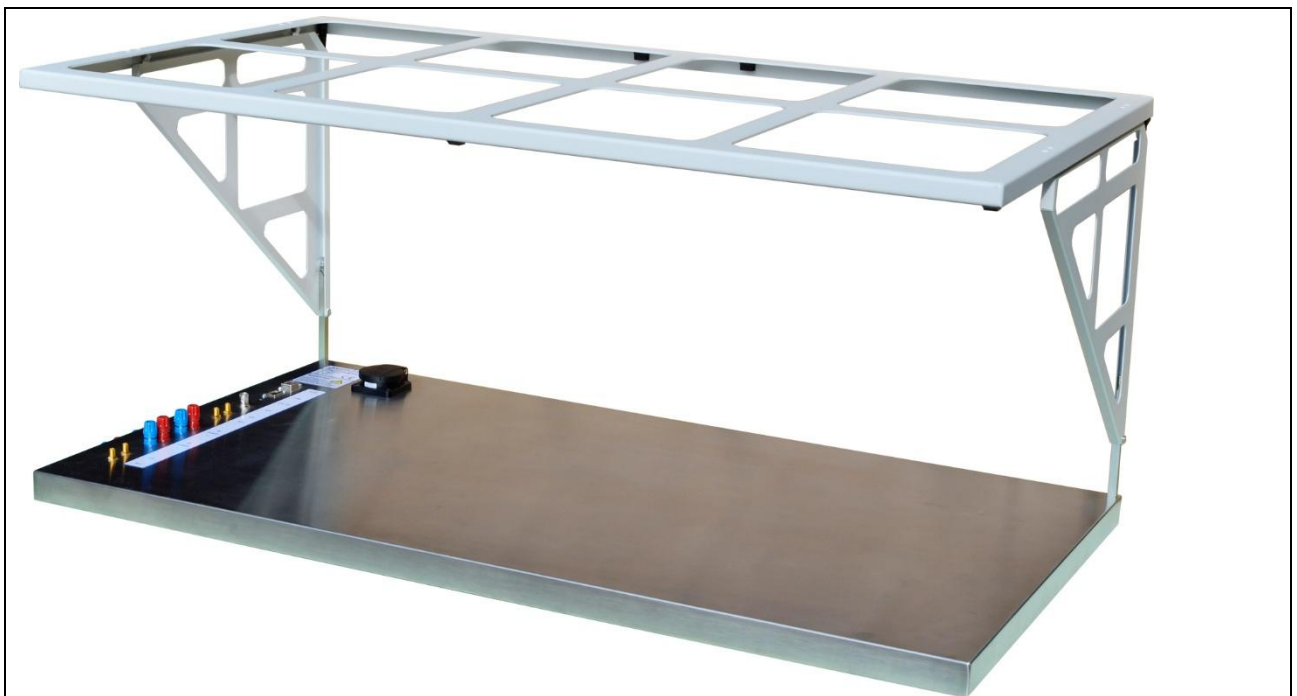
Figure 7 ZG 23-1 set up on the GP 23 ground plate
