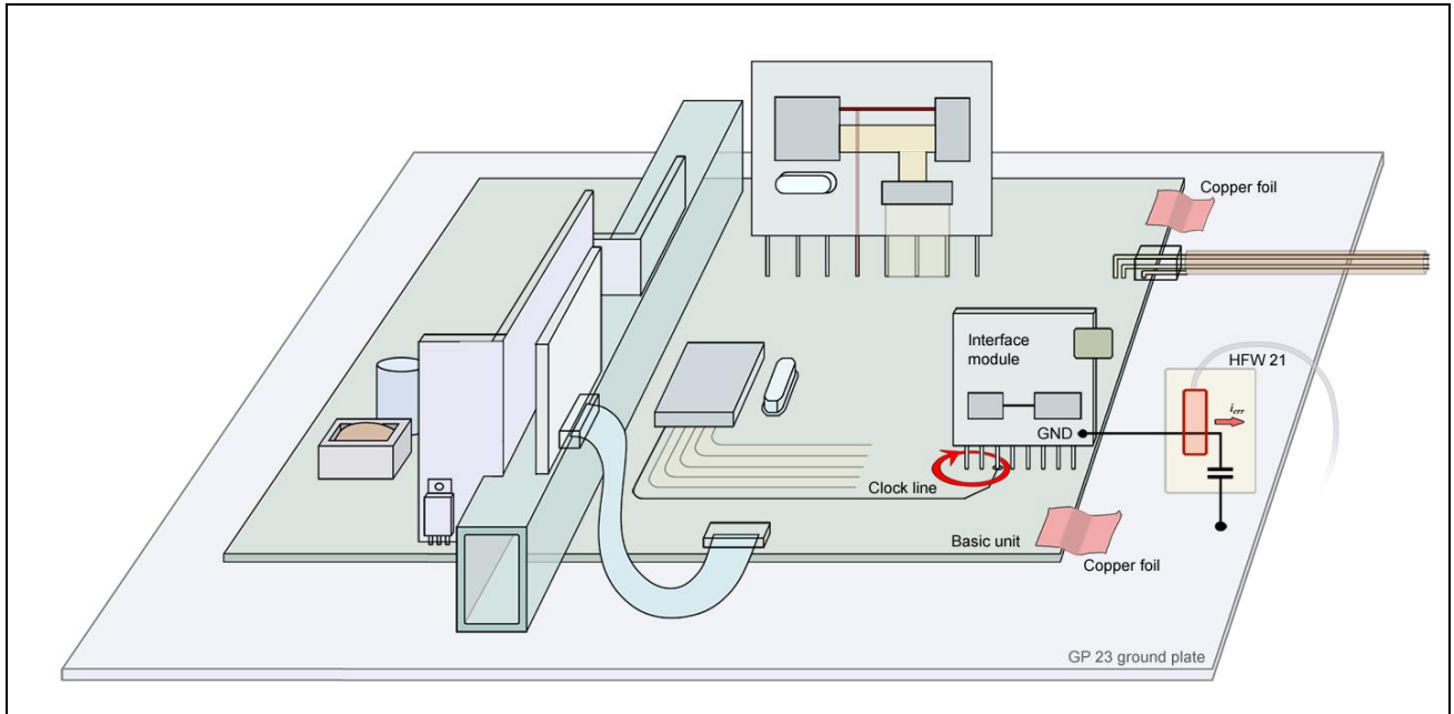
Figure 30 GND of the interface module connected to the COM output of the HFW 21
