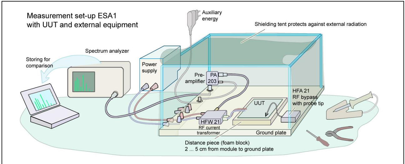
Figure 17 Measurement set-up ESA1 (schematic)
