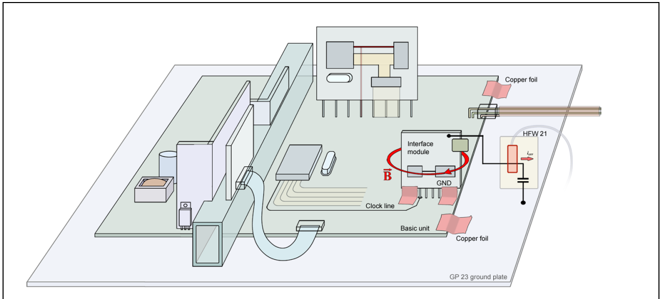
Figure 31 Evaluation of the modifications with the HFW 21
