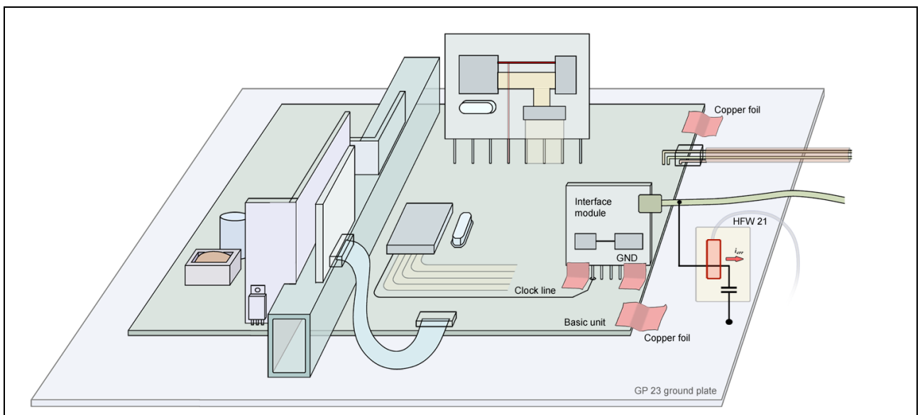
Figure 32 HFW 21 detects the voltage drop on the shield of the connected data cable
