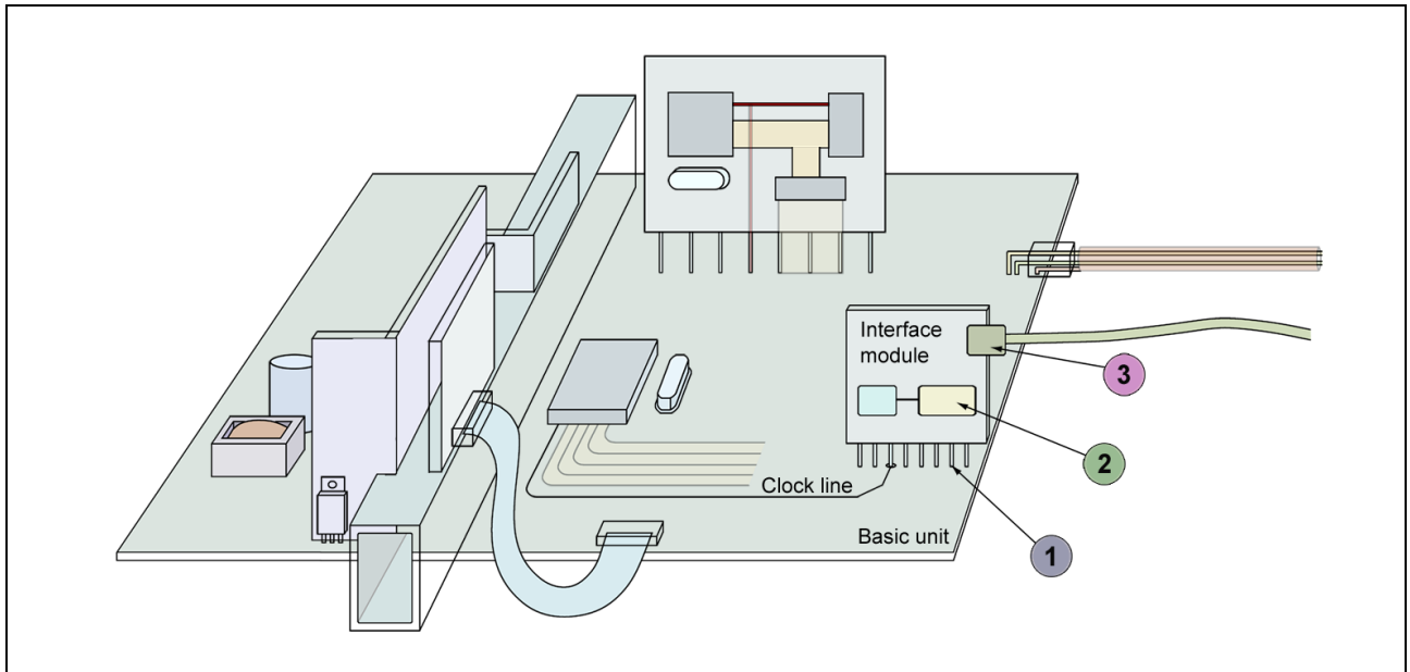
Figure 29 RF sources on the interface module
