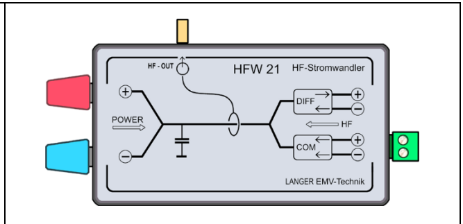
Figure 12 HFW 21 RF Current Transformer (schematic)
