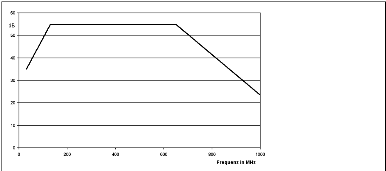
Figure 38 Approximate shield damping with the shielding tent closed
