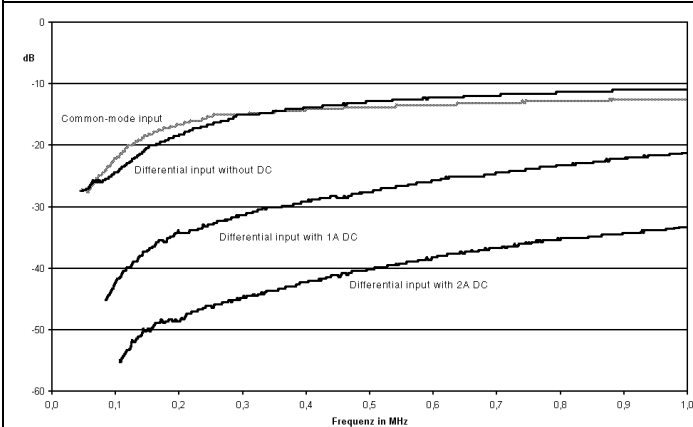
Figure 37 HFW 21 transfer performance
