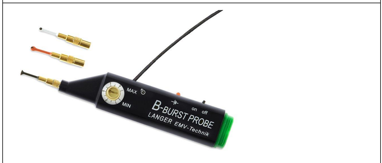
Figure 48: Magnetic field probe with exchangeable heads and an optical fibre from the S2 set.
