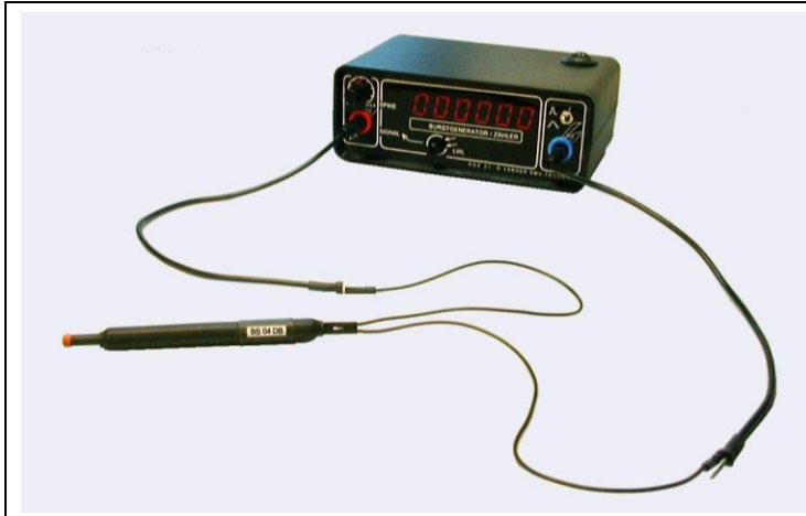
Figure 7: SGZ 21 with BS°04DB magnetic field source
