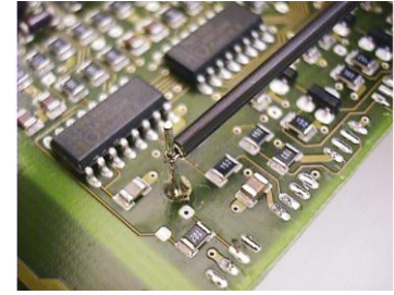
Figure 28: Prepare the ground layer by spot-facing, solder the contact pin in place, connect the generator cable to the contact pin with the micro-kleps and inject the disturbance current to ground via the conductor.
