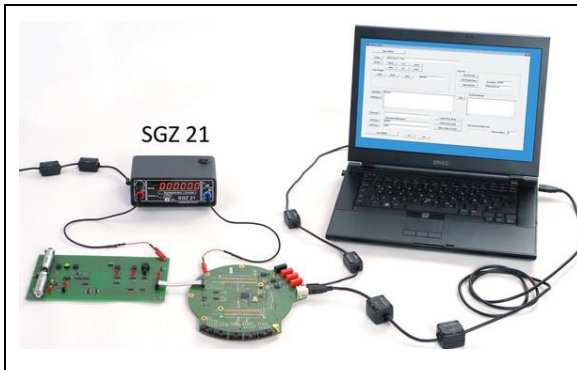
Figure 27: Injection of disturbance current via a two-pole connection and the connector of two modules. Contact is made to ground of each of the modules.
