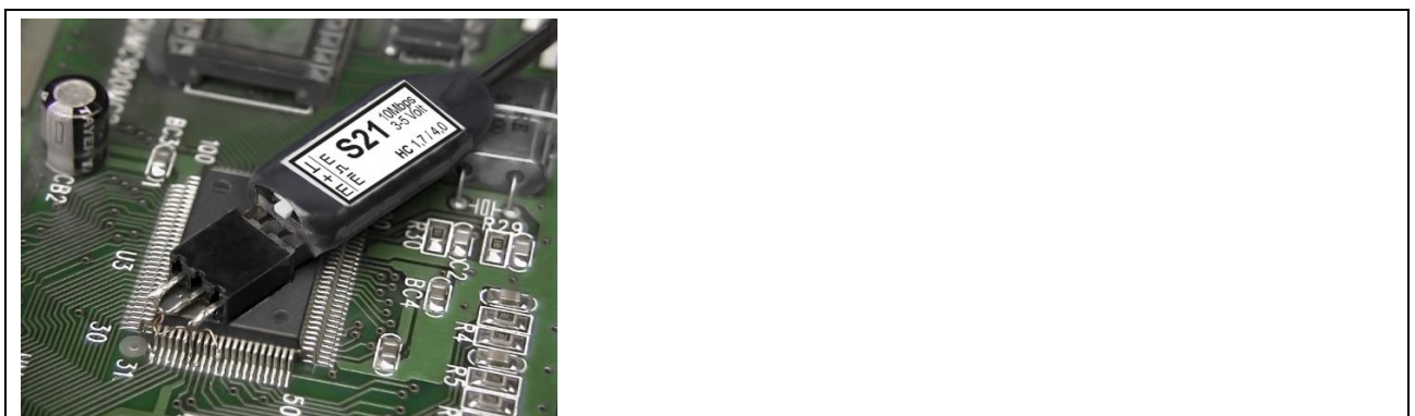
Figure 9: S21 sensor connected to an IC in the device under test, for example, via a three-pole socket.
