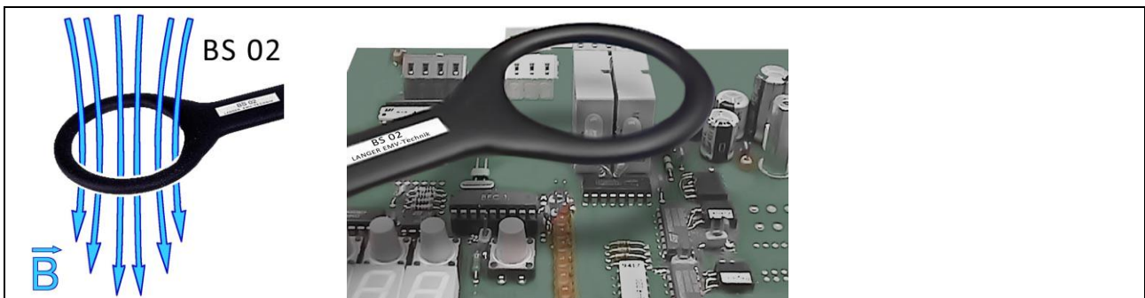
Figure 36: BS 02 field source with a large field beam to apply a magnetic field to conductor loops of around 10 cm.
