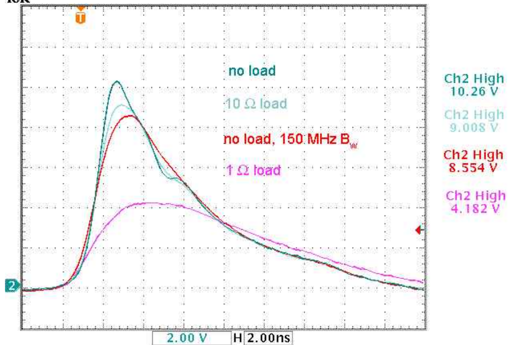
Pulsform (gemessen)
