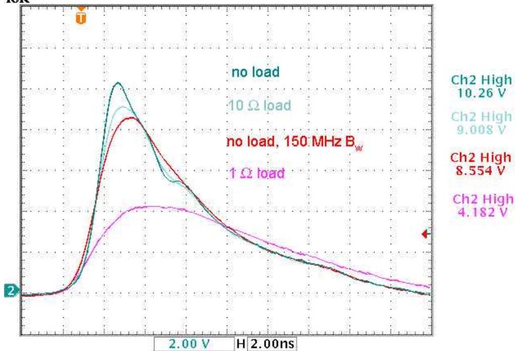
Pulsform (gemessen)
