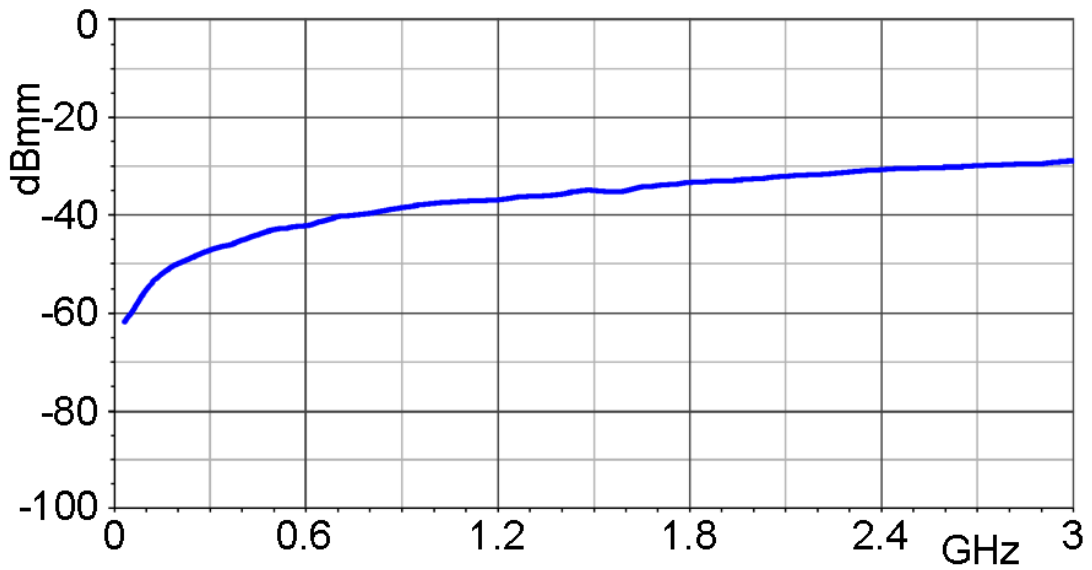
Frequenzgang
