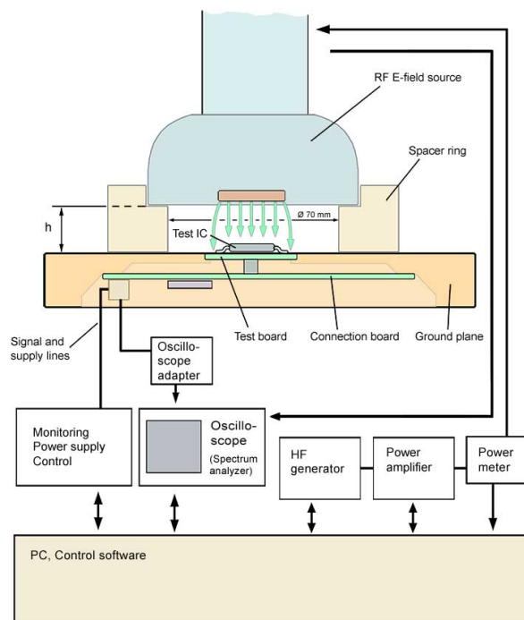
Measurement assembly with P1501 RF E-Field source (schematic)
