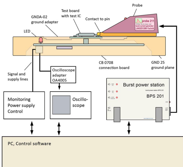
Measurement set up
