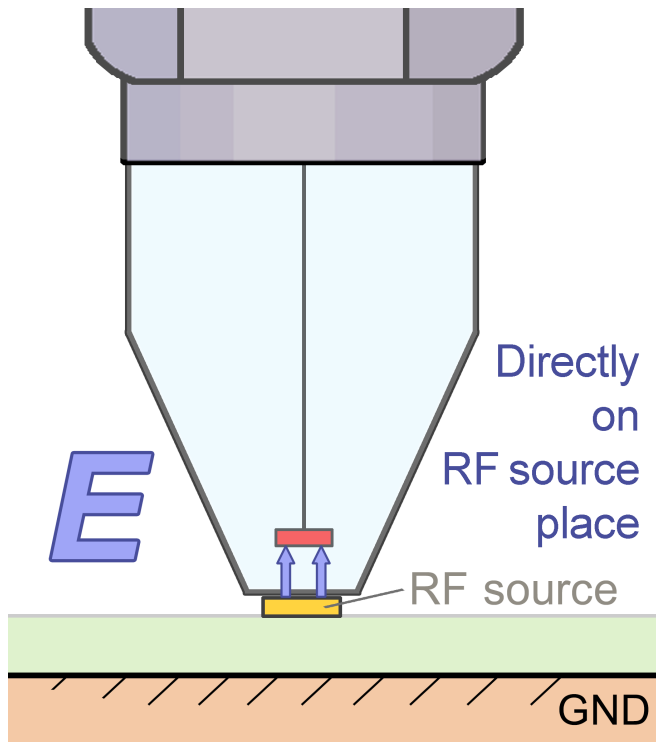
HR-E 40-1 E-field probe head
